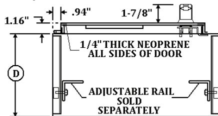
SECTION X-X WITH RELAY-RACK (OPTIONAL)
