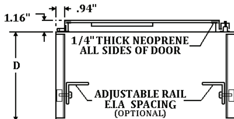
SECTION X-X WITH RELAY-RACK (OPTIONAL)
