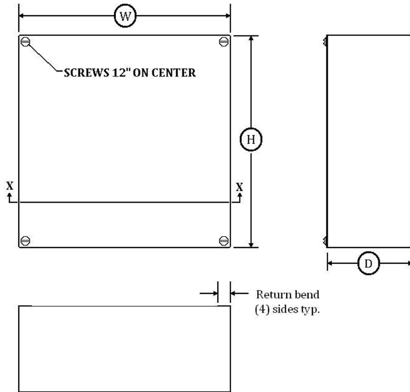
SECTION X-X (with cover removed)
