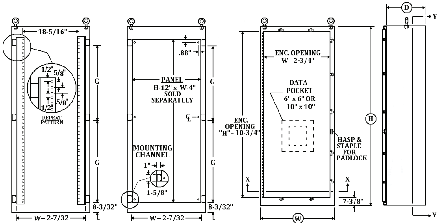
SECTION Y-Y WITH RELAY-RACK (OPTIONAL)
