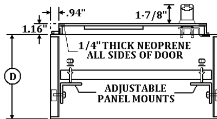
SECTION X-X WITH SUB-PANEL
