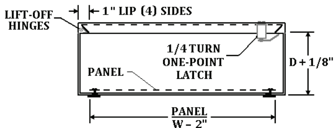
SECTION Y-Y
