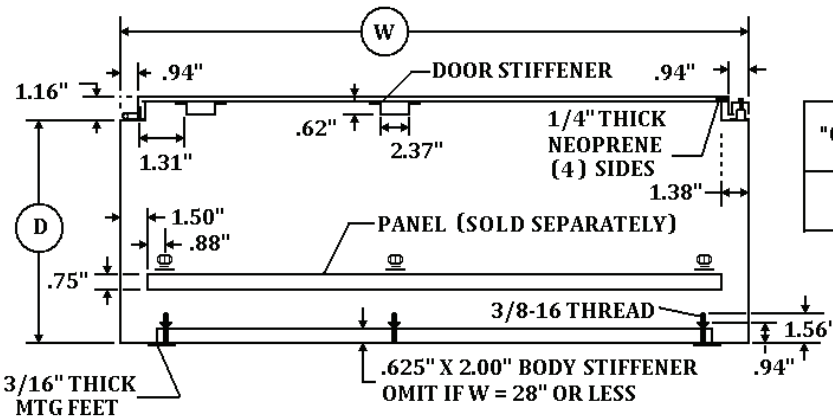
SECTION X-X
