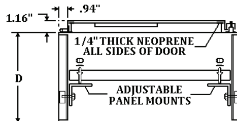
SECTION X-X WITH SUB-PANEL
